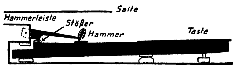
FIGURE 123. German Stossmechanik without escapement; del. Carmina Manger.
